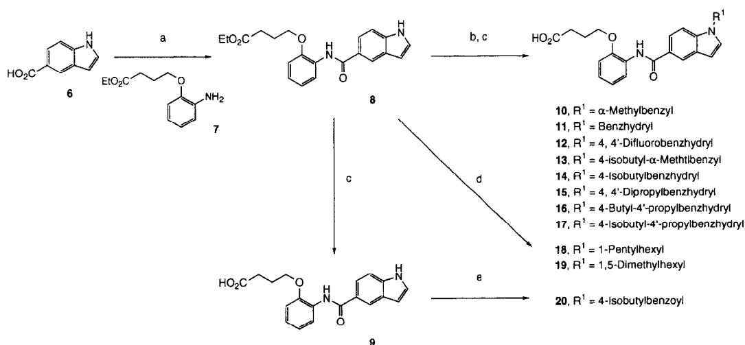
Scheme 1. (a) 2-Chloro-1-methylpyridinium iodide, \text{NBu}_3/\text{CH}_2\text{Cl}_2 ; (b) \text{R}^1\text{-Br} , t -BuOK/DMF; (c) NaOH/aq. EtOH; (d) \text{R}^1\text{-OTs} , KOH/DMSO; (e) t -BuOK, 4-isobutylbenzoyl chloride/DMF.
