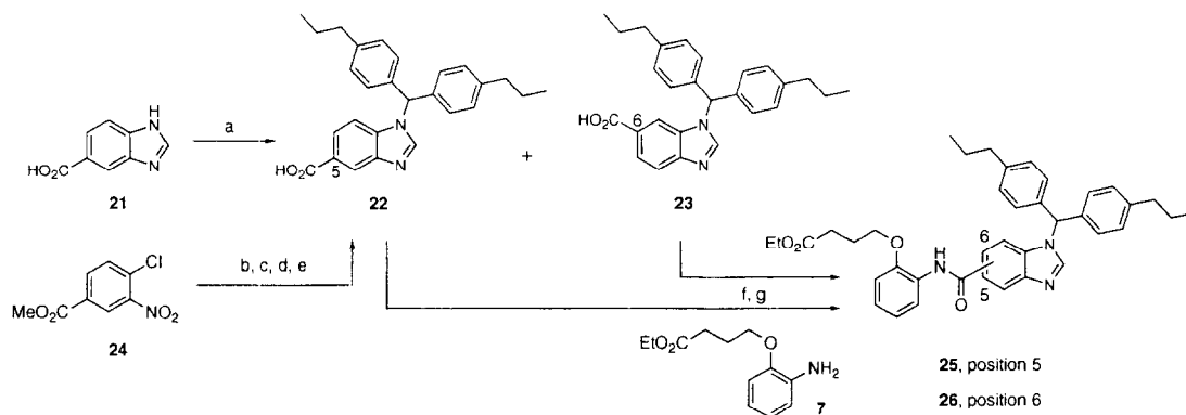
Scheme 2. (a) 4,4'-Dipropylbenzhydryl bromide, t -BuOK/DMF; (b) 4,4'-dipropylbenzhydryl amine/DMSO; (c) PtO 2 , H 2 /EtOH; (d) HC(OEt) 3 /HCO 2 H; (e) NaOH/aq. EtOH; (f) 2-chloro-1-methylpyridinium iodide, NBu 3 /CH 2 Cl 2 ; (g) NaOH/aq. EtOH.
