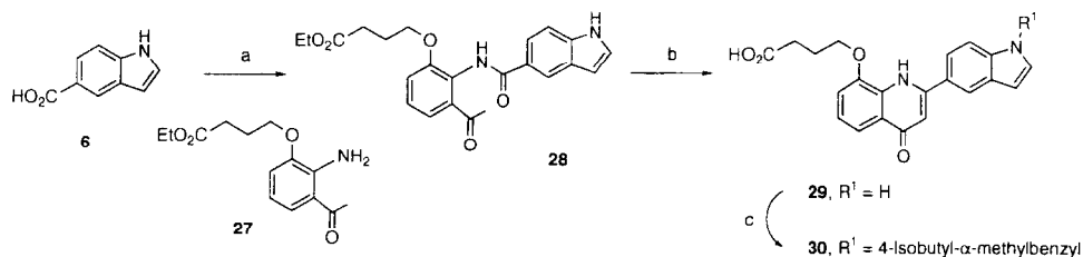
Scheme 3. (a) 2-Chloro-1-methylpyridinium iodide, NBu 3 /CH 2 Cl 2 ; (b) NaOMe/EtOH; (c) 4-isobutyl- \alpha -methylbenzyl bromide, t -BuOK/DMF.
